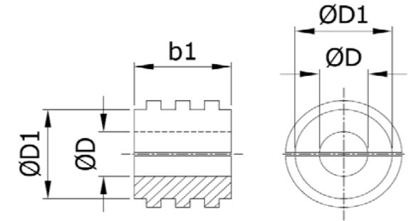
RUBBER INSERT
